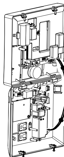
Figuur 3.6 – Power Supply Cable Connection
