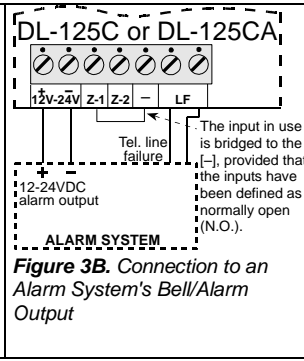
Figure 3A. Connection to an Alarm System with Constant Power Supply (Manual Dialing Stop)
