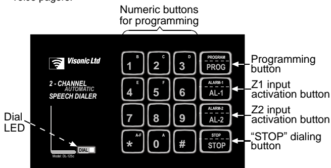
Figure 1. Front Panel
