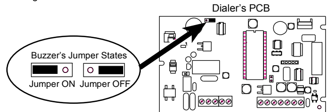
Figure 2.2. Moving Buzzer's Jumper to ON / OFF State
